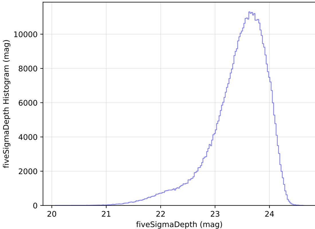
weather_cloudso14v3.4_10yrs WFD i band: fiveSigmaDepth Histogram
