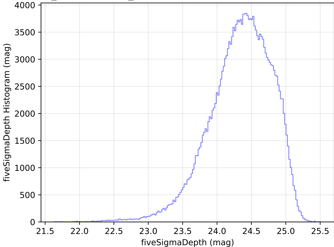
weather_cloudso14v3.4_10yrs WFD g band: fiveSigmaDepth Histogram
