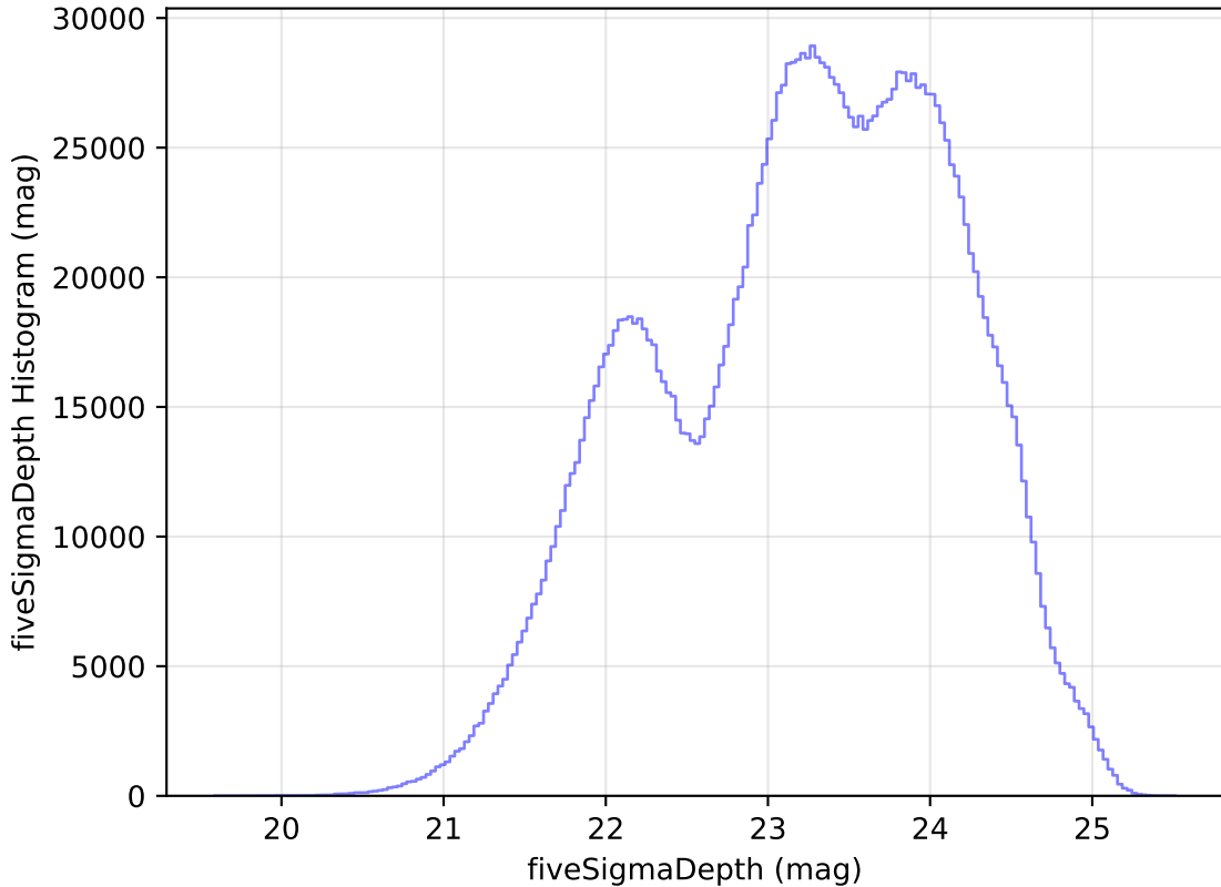
weather_cloudso14v3.4_10yrs WFD all bands: fiveSigmaDepth Histogram
