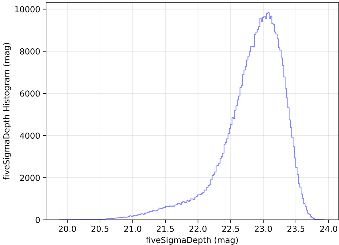
weather_cloudso14v3.4_10yrs All sky z band: fiveSigmaDepth Histogram
