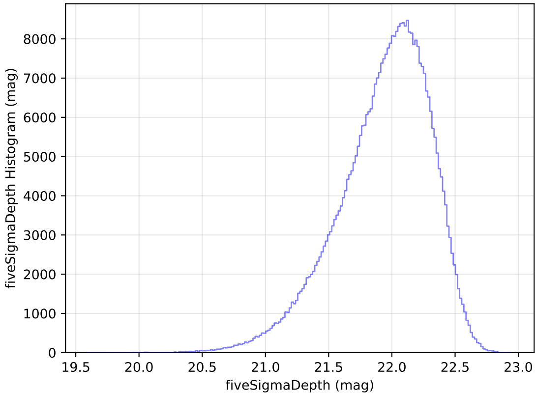
weather_cloudso14v3.4_10yrs All sky y band: fiveSigmaDepth Histogram
