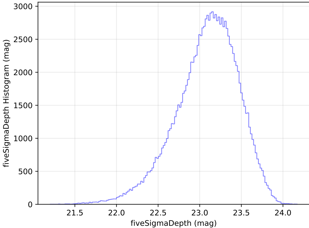
weather_cloudso14v3.4_10yrs All sky u band: fiveSigmaDepth Histogram
