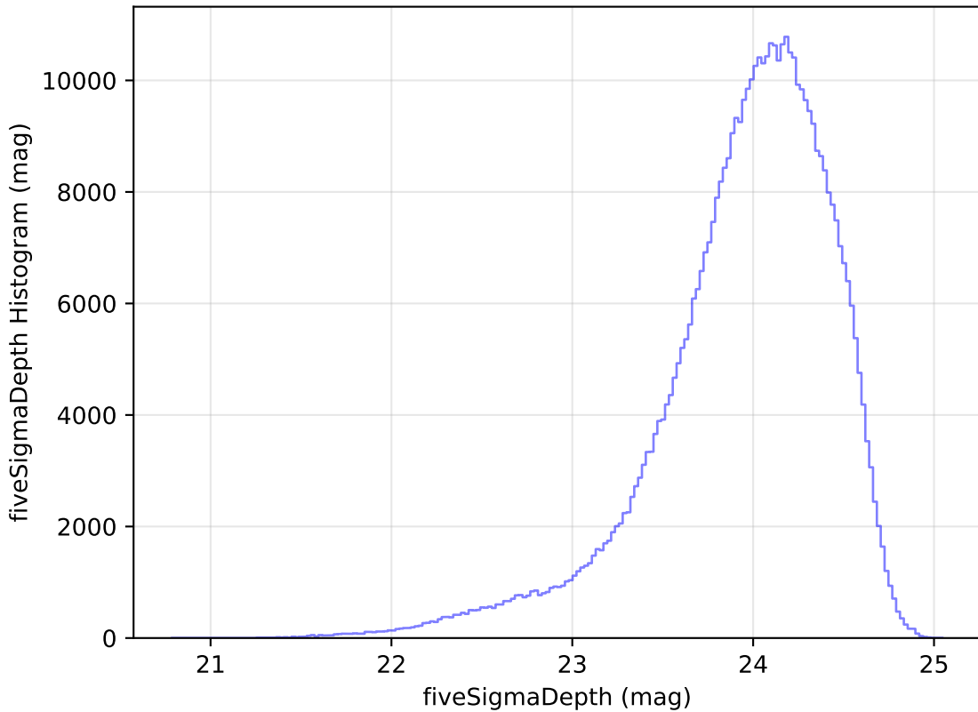
weather_cloudso14v3.4_10yrs All sky r band: fiveSigmaDepth Histogram
