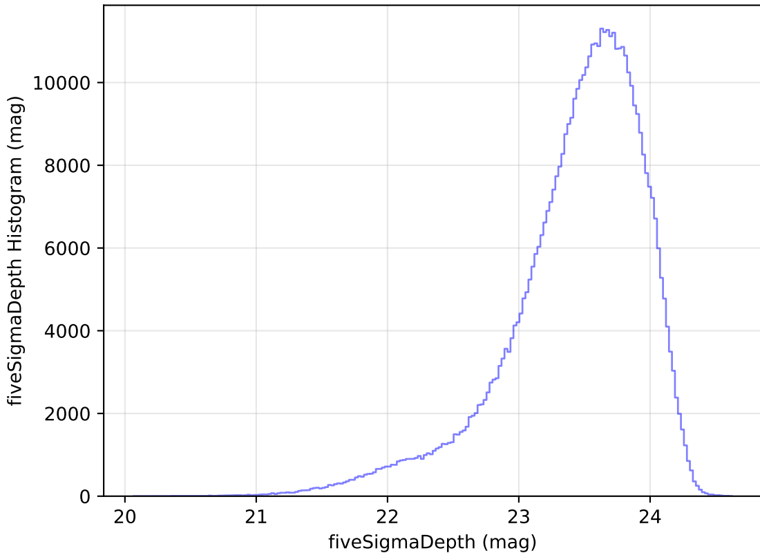
weather_cloudso14v3.4_10yrs All sky i band: fiveSigmaDepth Histogram
