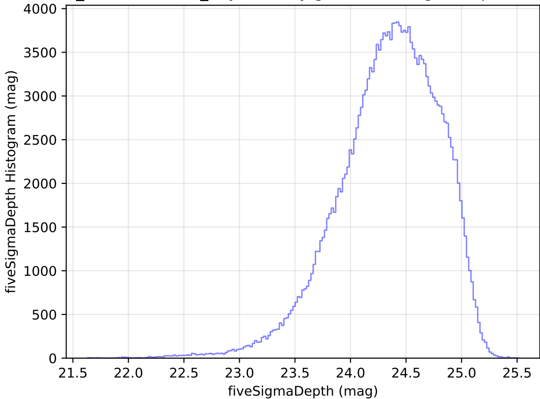
weather_cloudso14v3.4_10yrs All sky g band: fiveSigmaDepth Histogram
