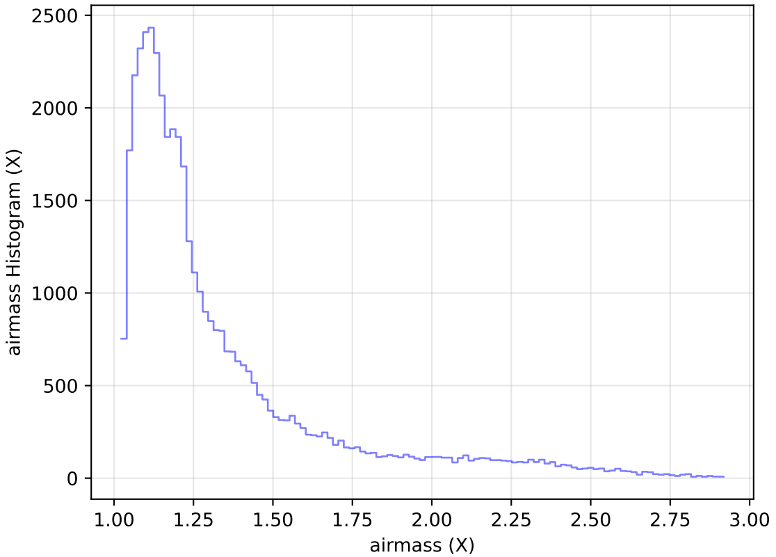
weather_cloudso14v3.4_10yrs Yr 1 z band: airmass Histogram
