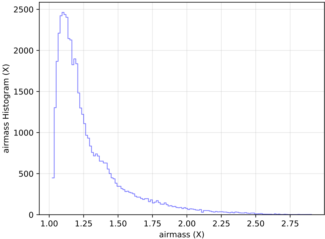
weather_cloudso14v3.4_10yrs Yr 1 y band: airmass Histogram
