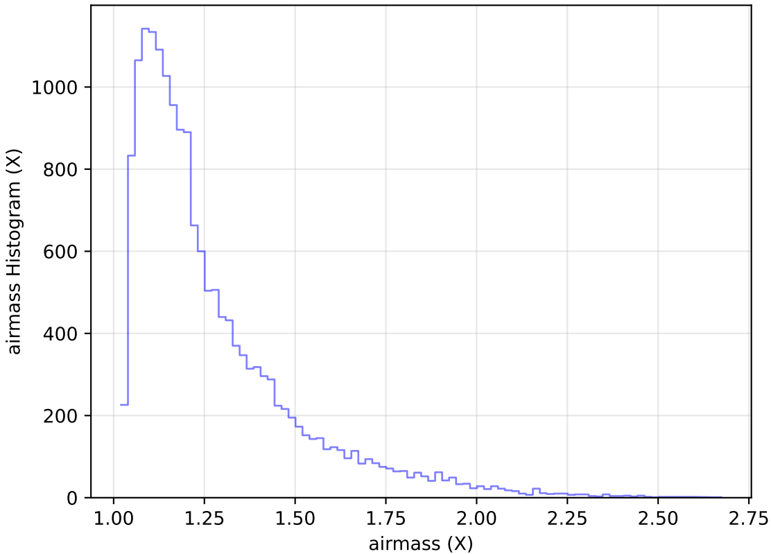
weather_cloudso14v3.4_10yrs Yr 1 u band: airmass Histogram
