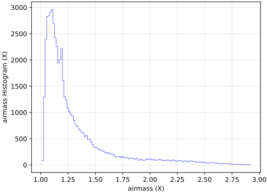
weather_cloudso14v3.4_10yrs Yr 1 i band: airmass Histogram
