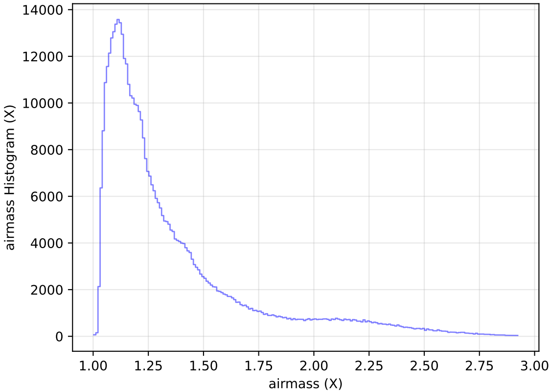
weather_cloudso14v3.4_10yrs WFD z band: airmass Histogram
