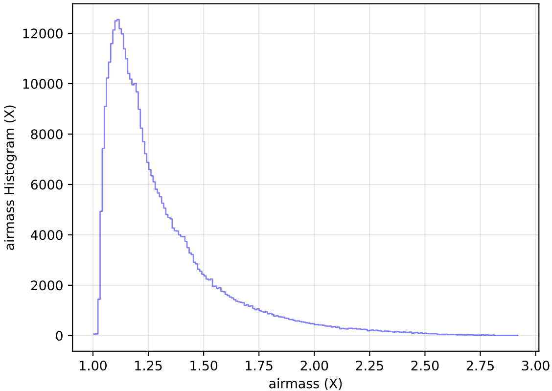
weather_cloudso14v3.4_10yrs WFD y band: airmass Histogram
