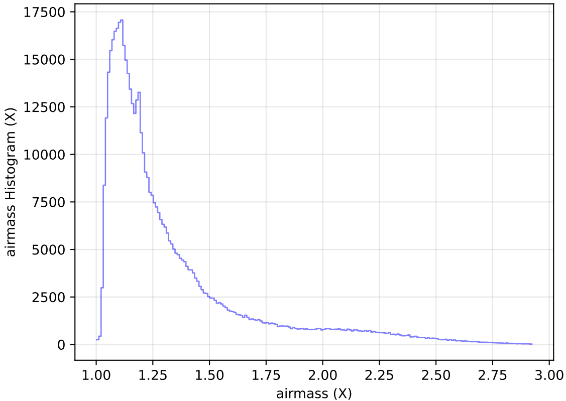
weather_cloudso14v3.4_10yrs WFD i band: airmass Histogram
