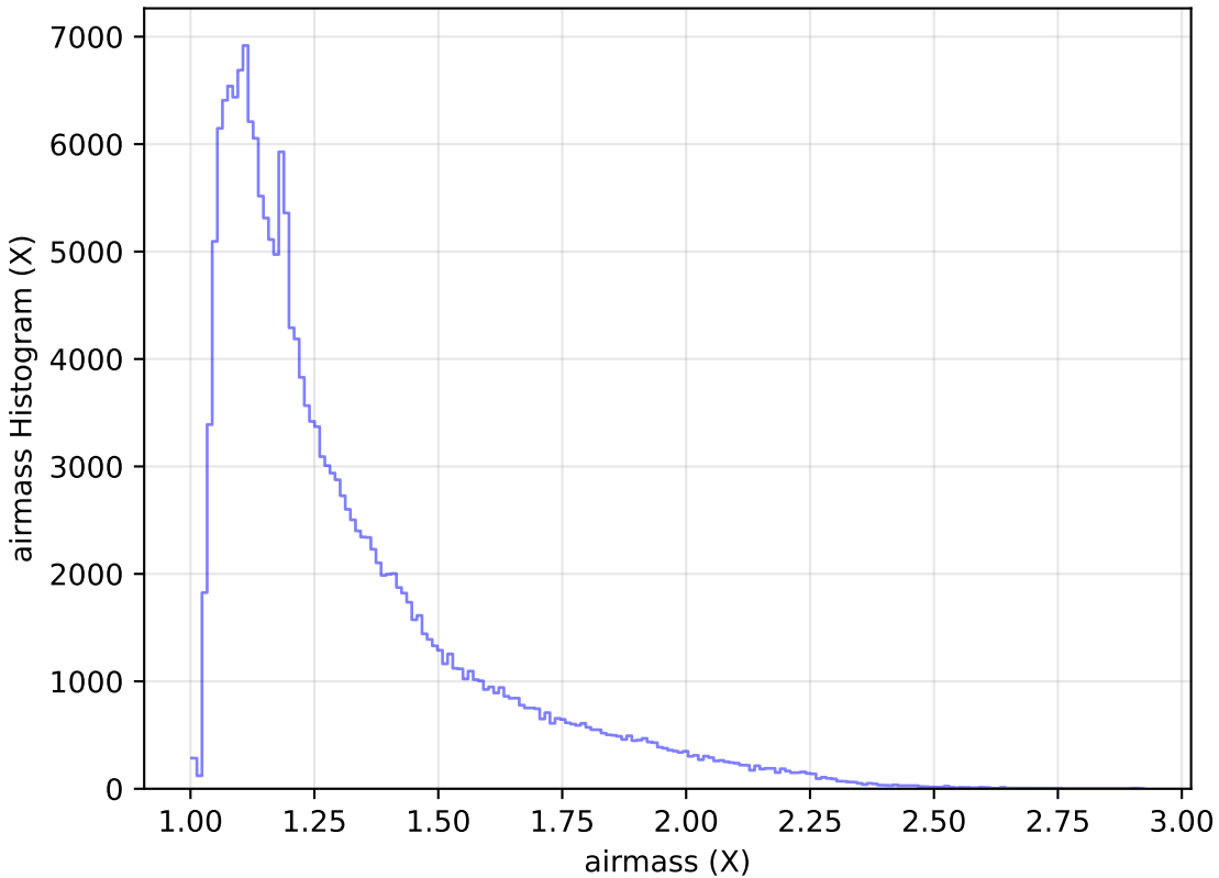
weather_cloudso14v3.4_10yrs WFD g band: airmass Histogram
