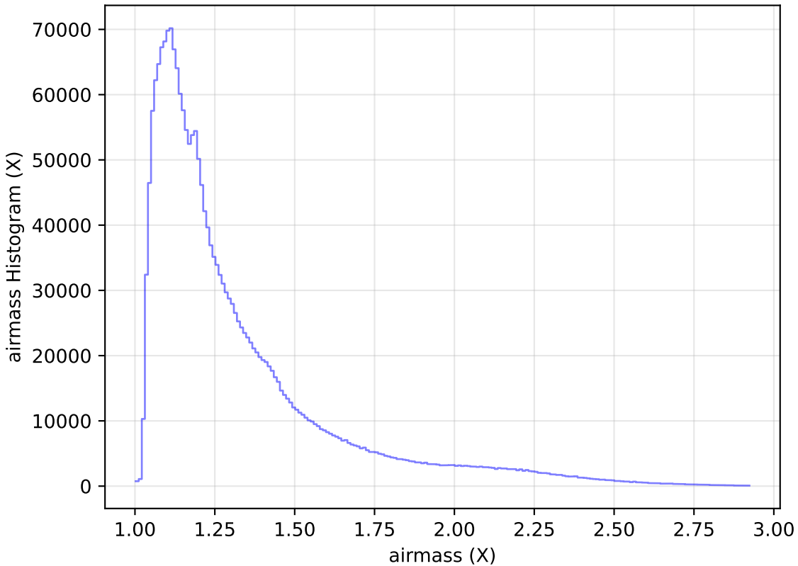
weather_cloudso14v3.4_10yrs WFD all bands: airmass Histogram
