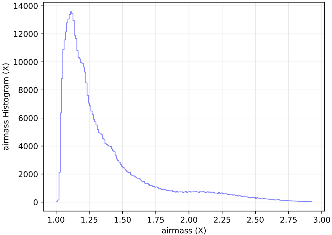
weather_cloudso14v3.4_10yrs All sky z band: airmass Histogram
