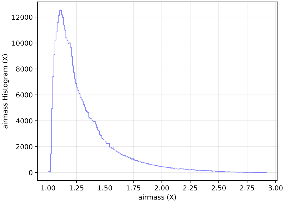
weather_cloudso14v3.4_10yrs All sky y band: airmass Histogram
