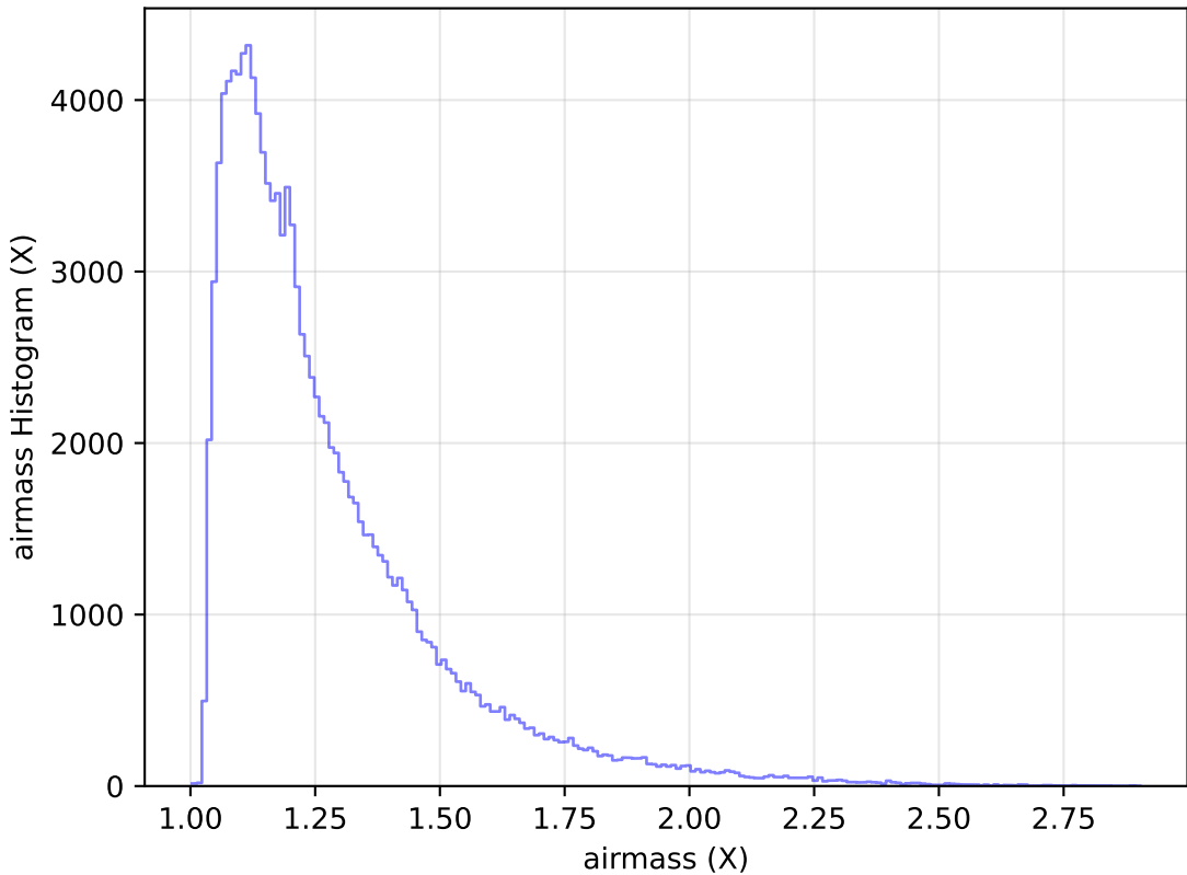
weather_cloudso14v3.4_10yrs All sky u band: airmass Histogram
