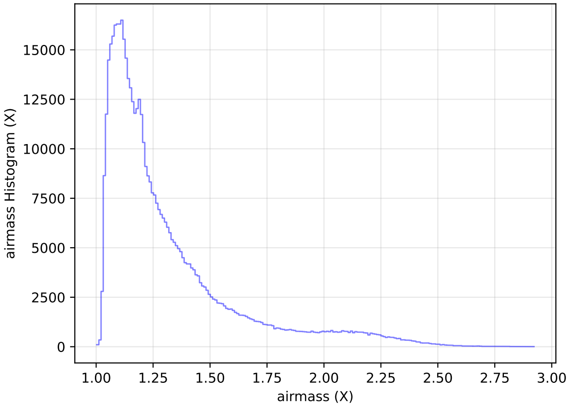
weather_cloudso14v3.4_10yrs All sky r band: airmass Histogram
