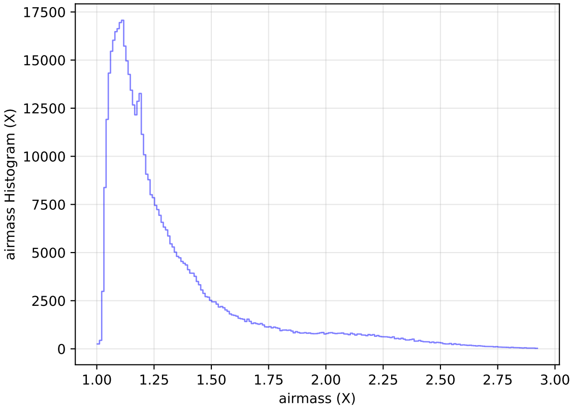
weather_cloudso14v3.4_10yrs All sky i band: airmass Histogram
