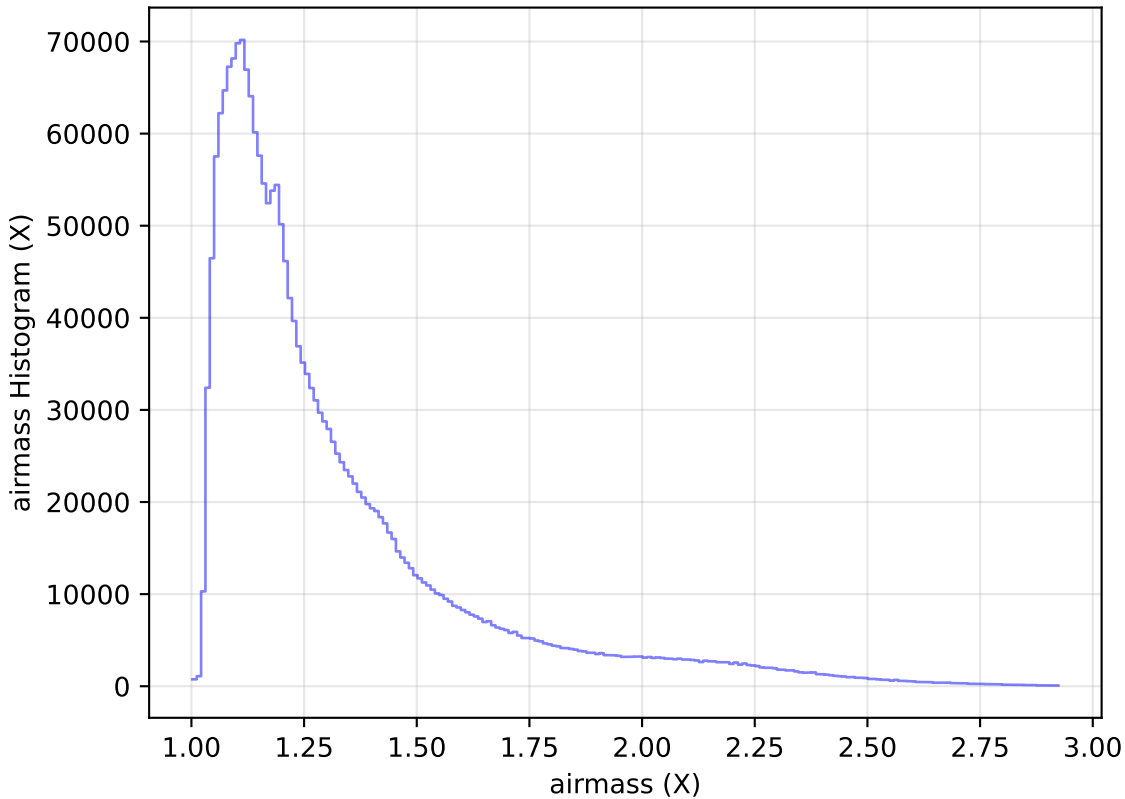
weather_cloudso14v3.4_10yrs All sky all bands: airmass Histogram
