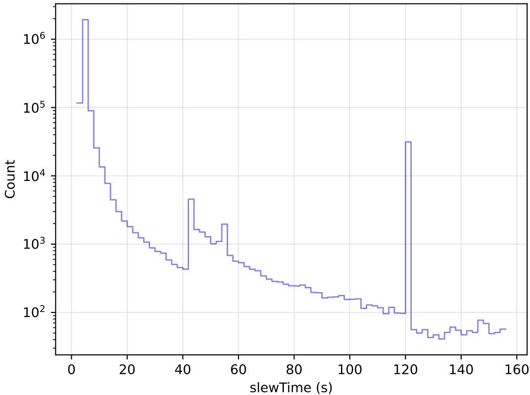
weather_cloudso14v3.4_10yrs All visits: Slew Time Histogram
