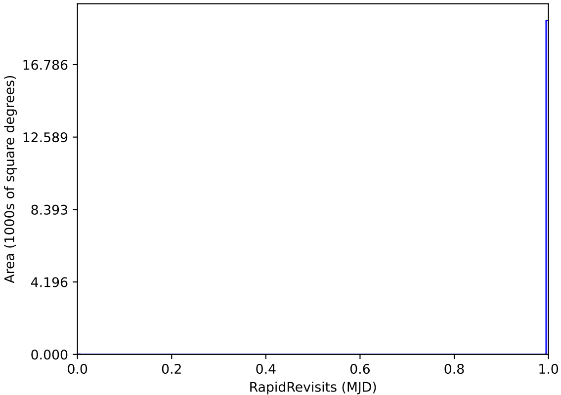
weather_cloudso14v3.4_10yrs WFD: RapidRevisits
