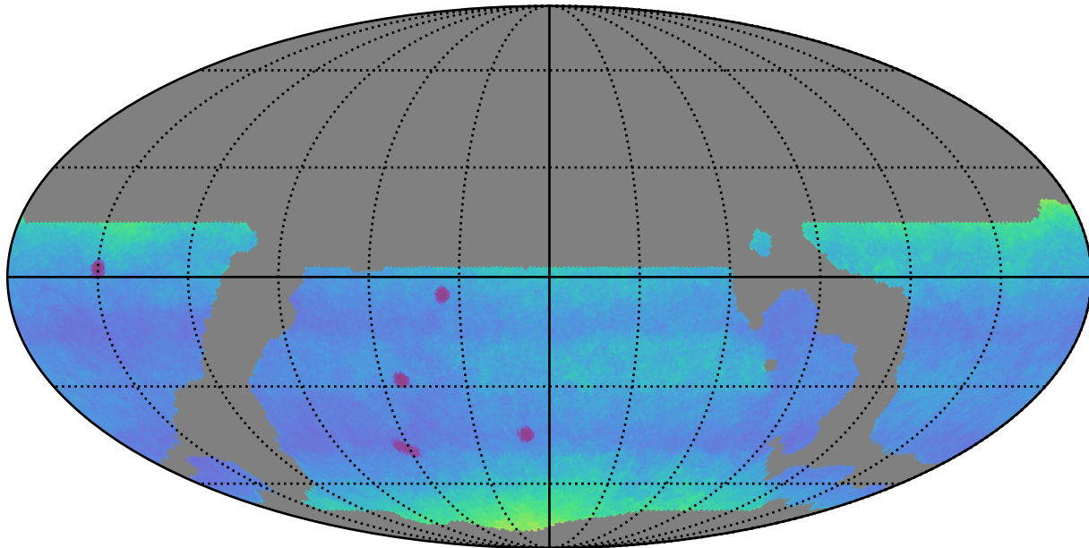
weather_cloudso14v3.4_10yrs WFD: Proper Motion Uncert @ 24.0
