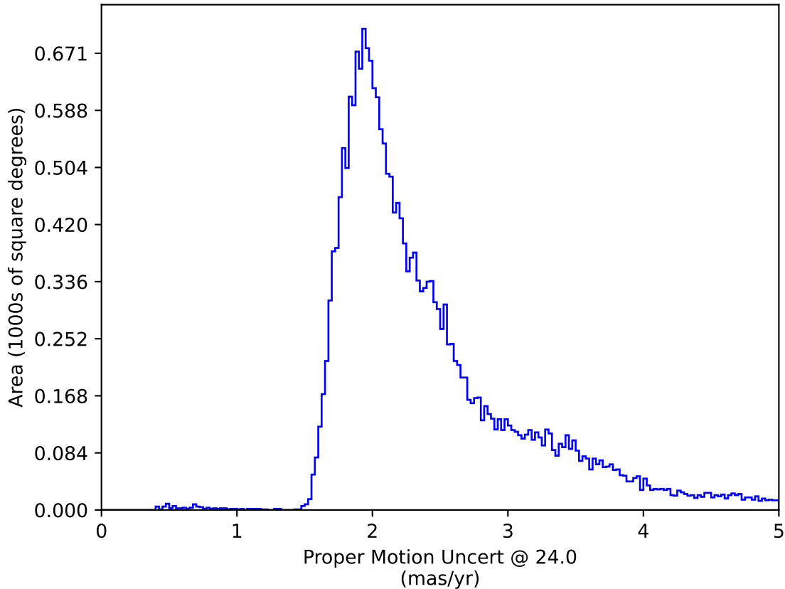
weather_cloudso14v3.4_10yrs All sky: Proper Motion Uncert @ 24.0
