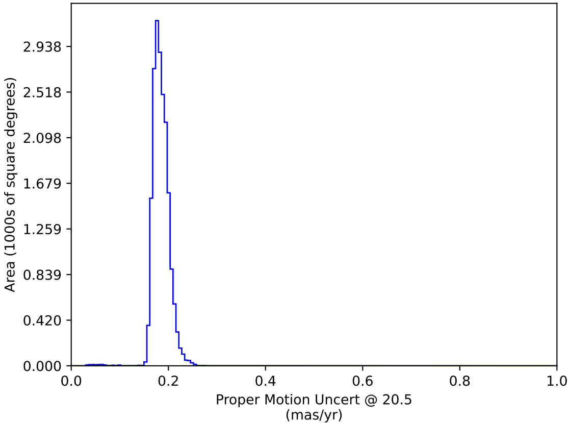
weather_cloudso14v3.4_10yrs WFD: Proper Motion Uncert @ 20.5
