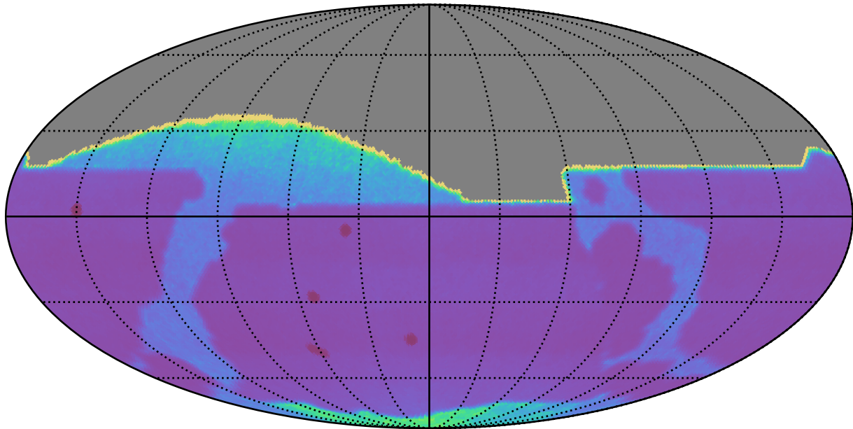
weather_cloudso14v3.4_10yrs All sky: Proper Motion Uncert @ 20.5
