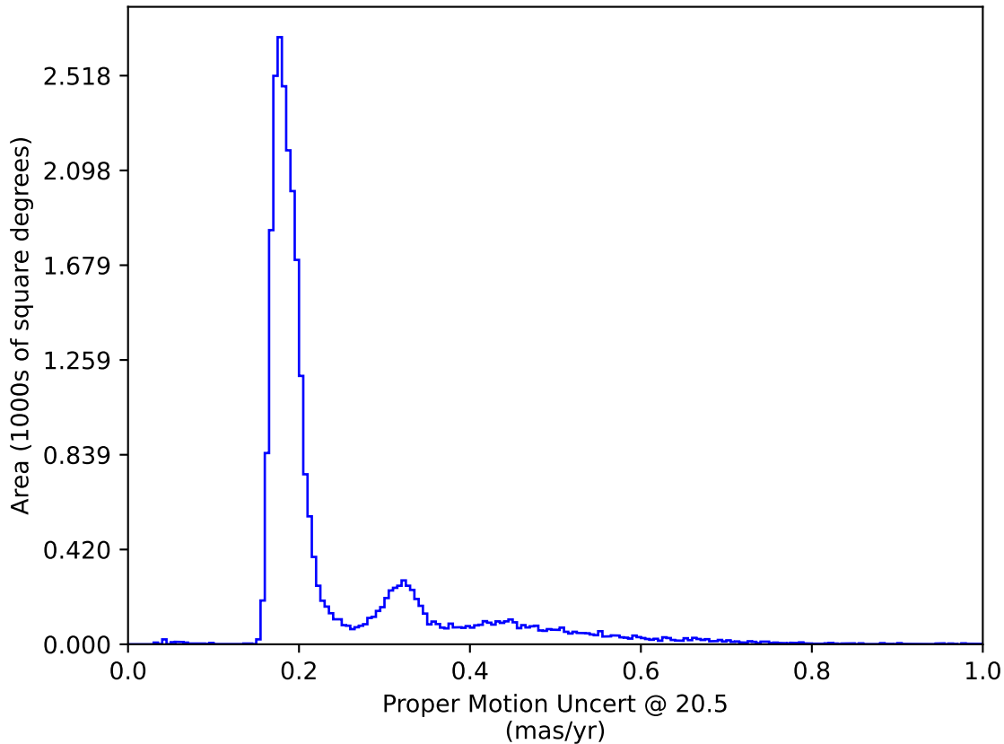
weather_cloudso14v3.4_10yrs All sky: Proper Motion Uncert @ 20.5
