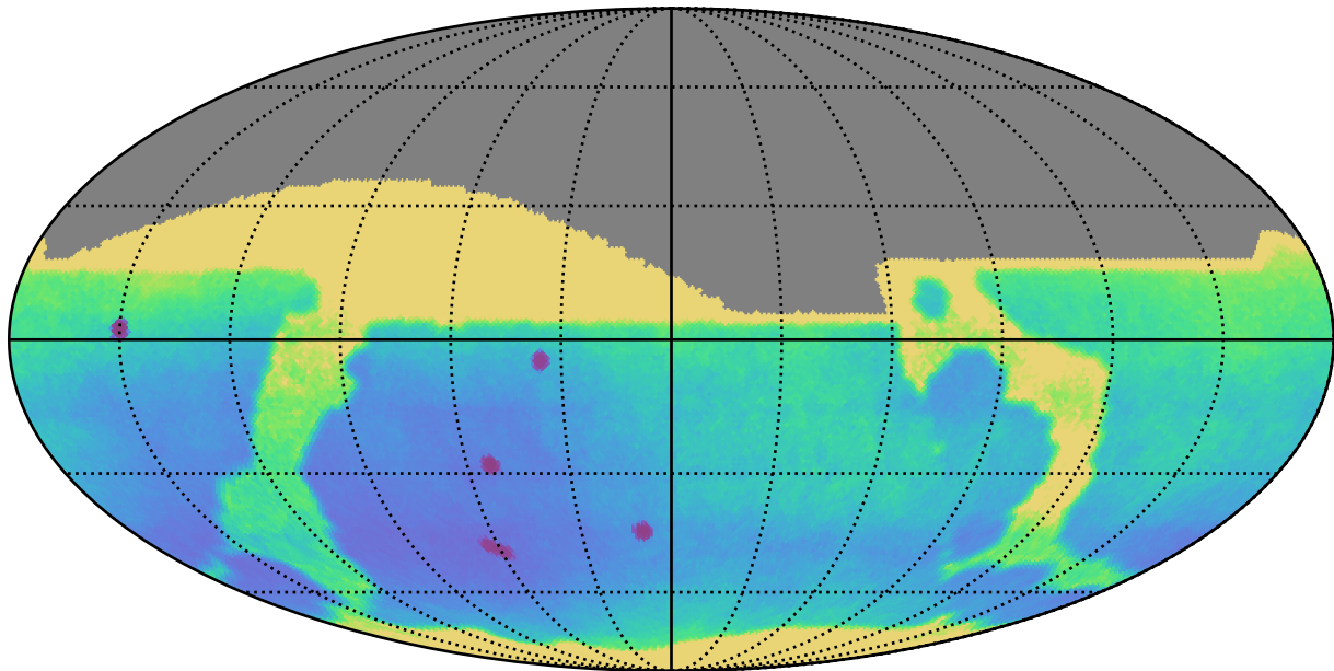
weather_cloudso14v3.4_10yrs All sky: Parallax Uncert @ 24.0
