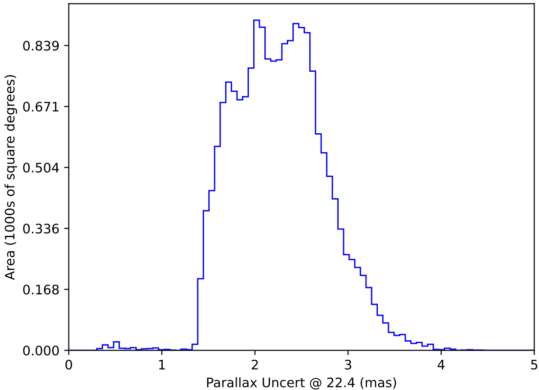
weather_cloudso14v3.4_10yrs WFD: Parallax Uncert @ 22.4
