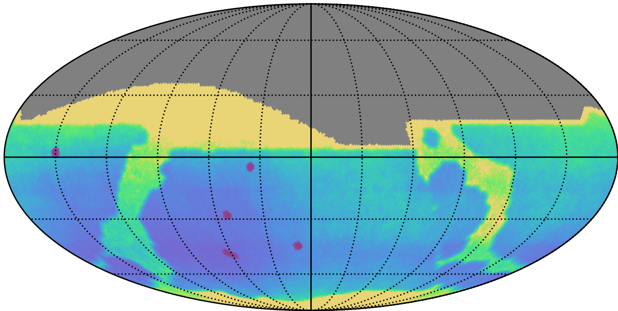
weather_cloudso14v3.4_10yrs All sky: Parallax Uncert @ 22.4
