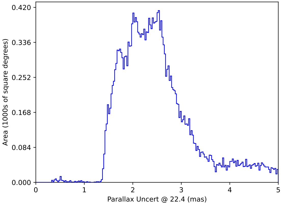
weather_cloudso14v3.4_10yrs All sky: Parallax Uncert @ 22.4
