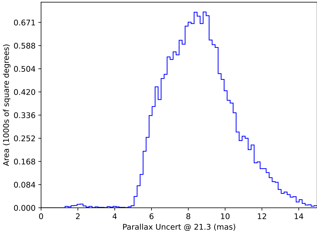
weather_cloudso14v3.4_10yrs WFD y band only: Parallax Uncert @ 21.3
