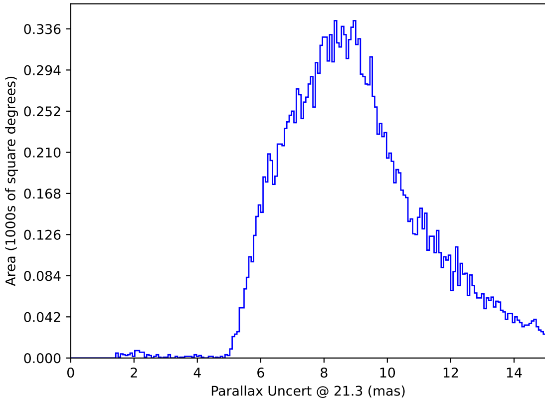
weather_cloudso14v3.4_10yrs All sky y band only: Parallax Uncert @ 21.3
