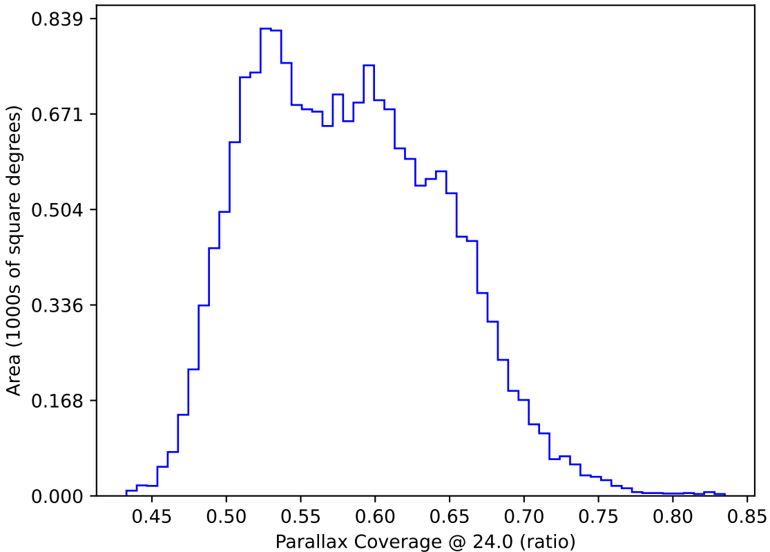
weather_cloudso14v3.4_10yrs WFD: Parallax Coverage @ 24.0
