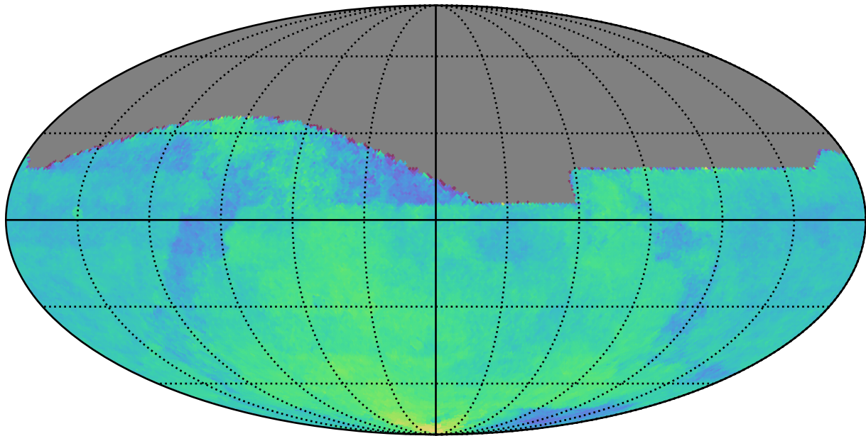
weather_cloudso14v3.4_10yrs All sky: Parallax Coverage @ 24.0
