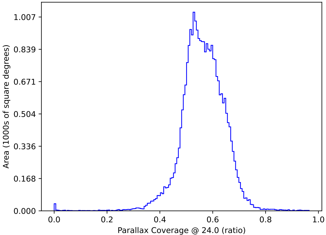
weather_cloudso14v3.4_10yrs All sky: Parallax Coverage @ 24.0
