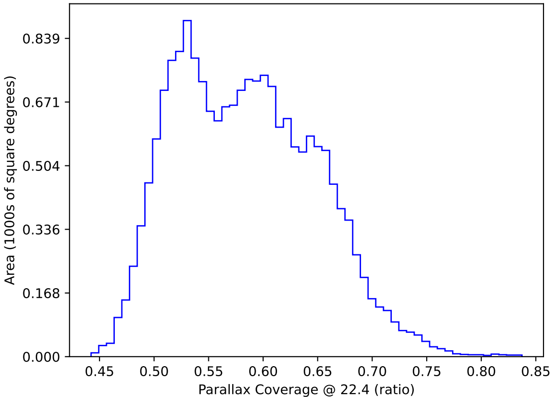
weather_cloudso14v3.4_10yrs WFD: Parallax Coverage @ 22.4
