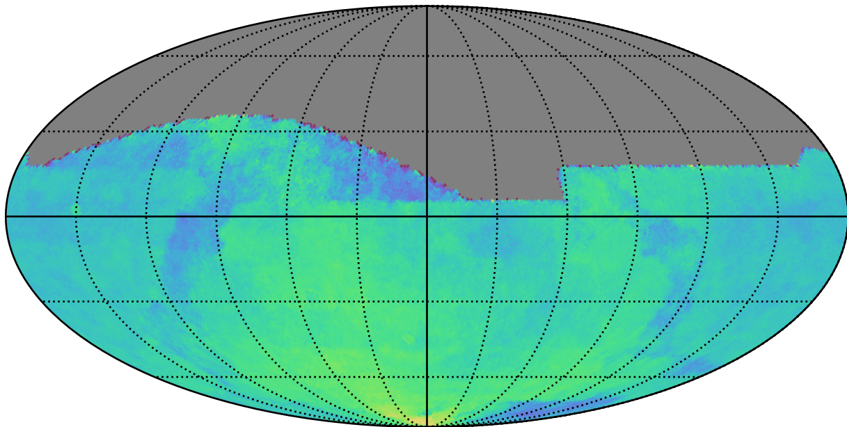
weather_cloudso14v3.4_10yrs All sky: Parallax Coverage @ 22.4
