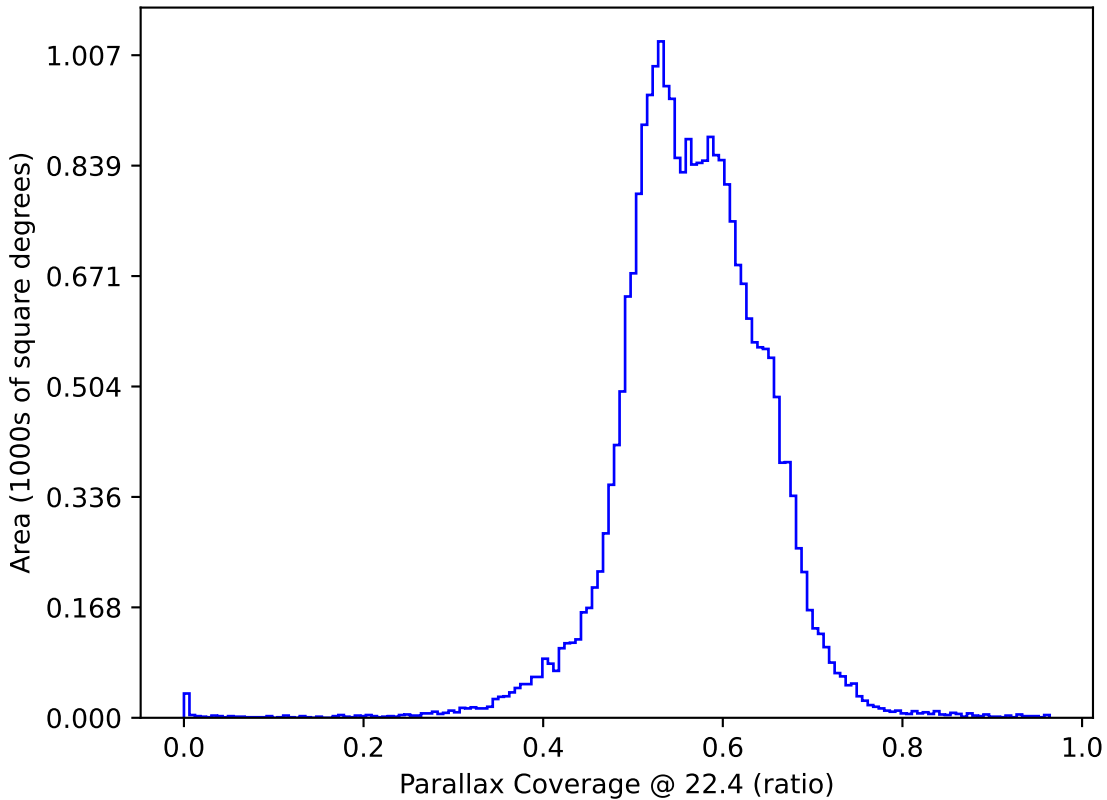
weather_cloudso14v3.4_10yrs All sky: Parallax Coverage @ 22.4
