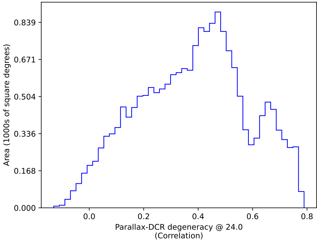
weather_cloudso14v3.4_10yrs WFD: Parallax-DCR degeneracy @ 24.0
