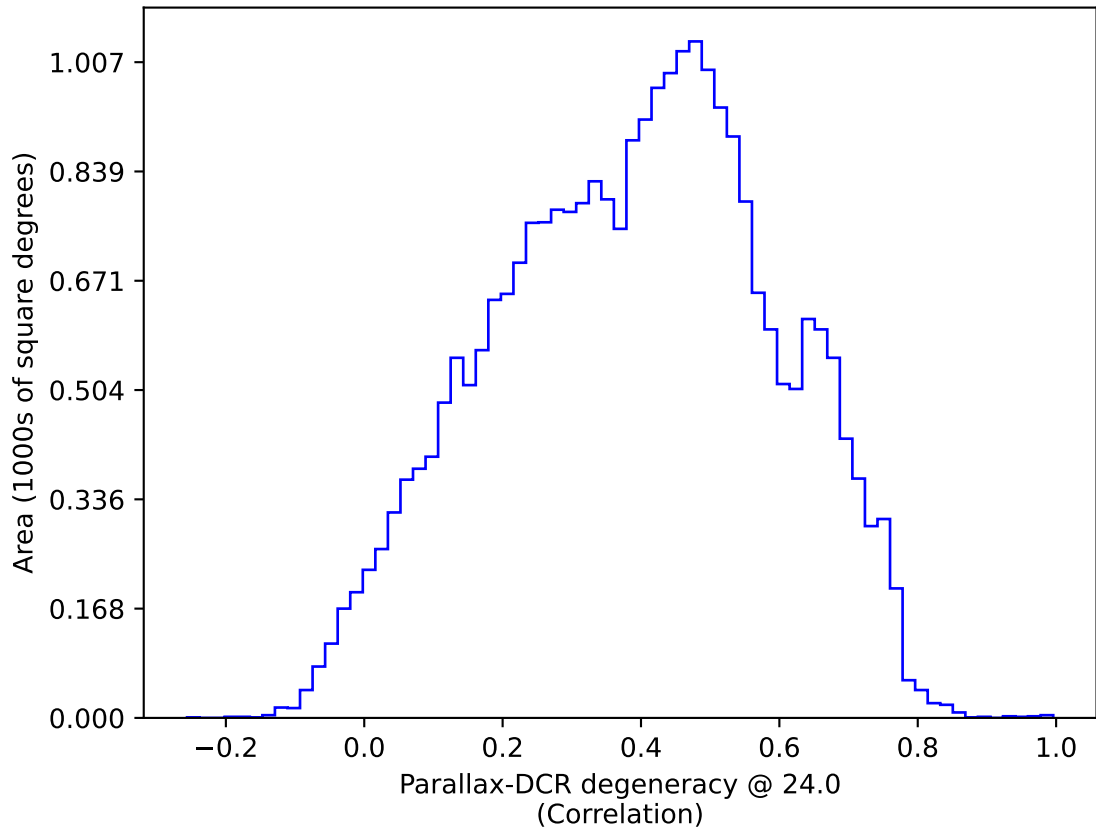
weather_cloudso14v3.4_10yrs All sky: Parallax-DCR degeneracy @ 24.0
