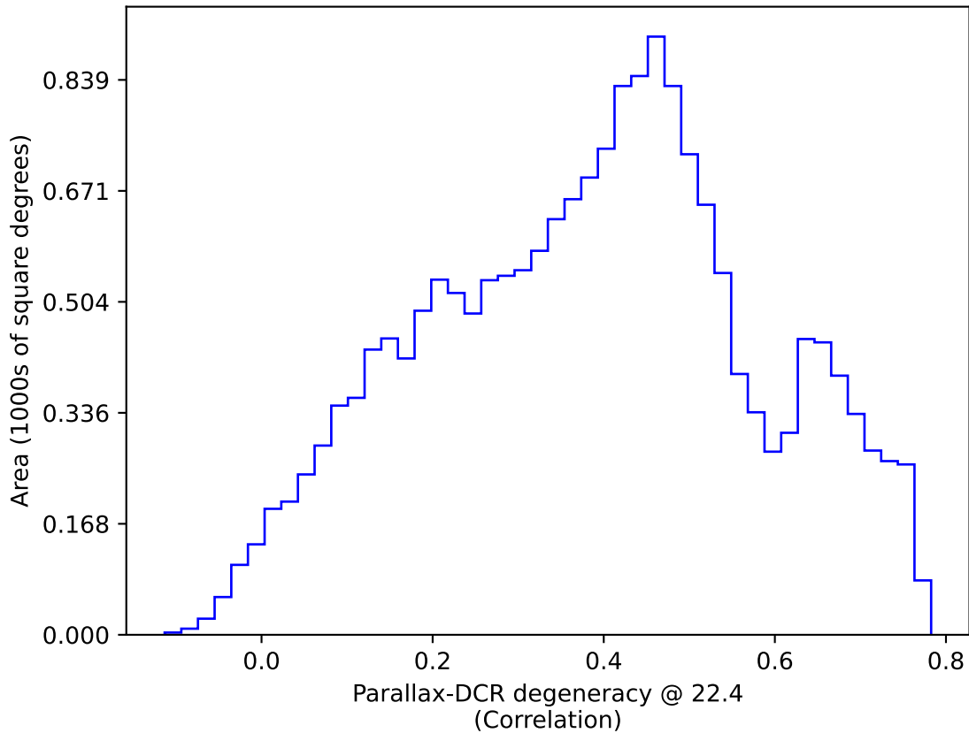
weather_cloudso14v3.4_10yrs WFD: Parallax-DCR degeneracy @ 22.4
