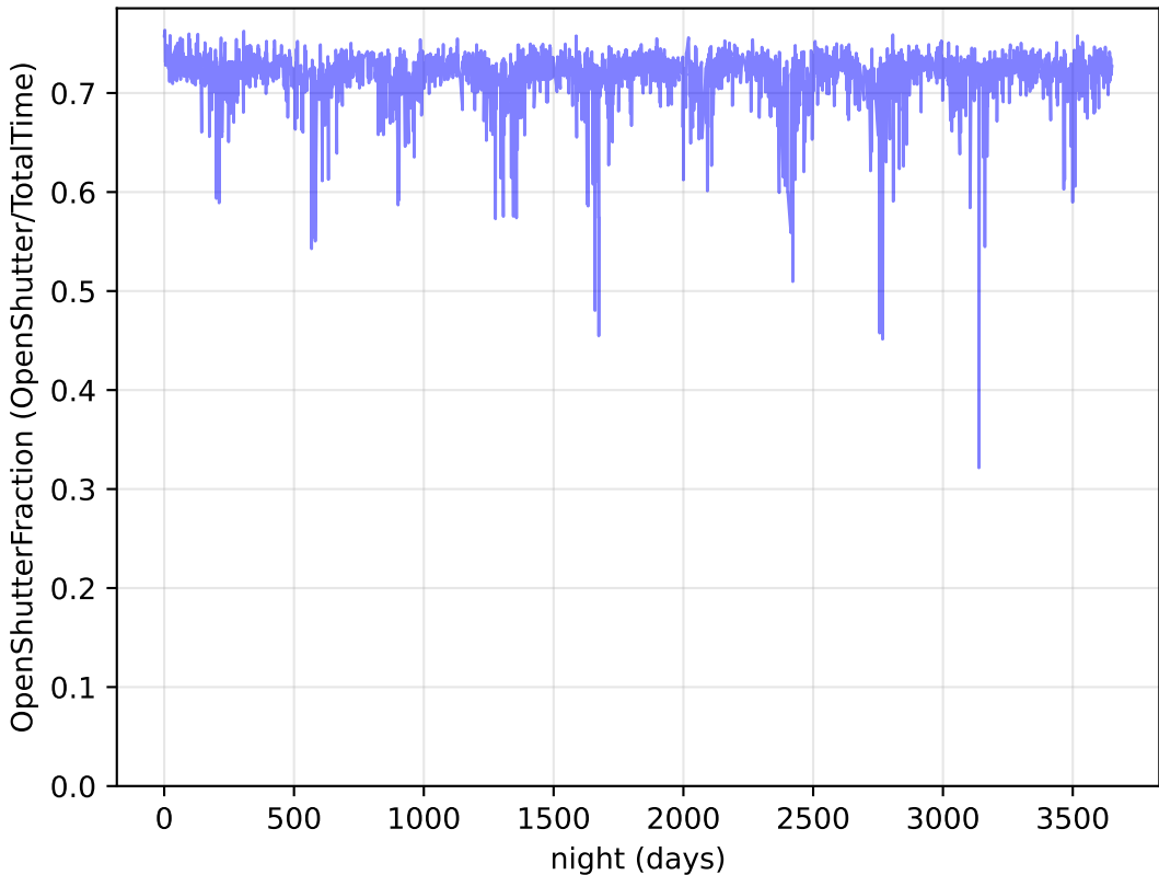
weather_cloudso14v3.4_10yrs Per night: OpenShutterFraction
