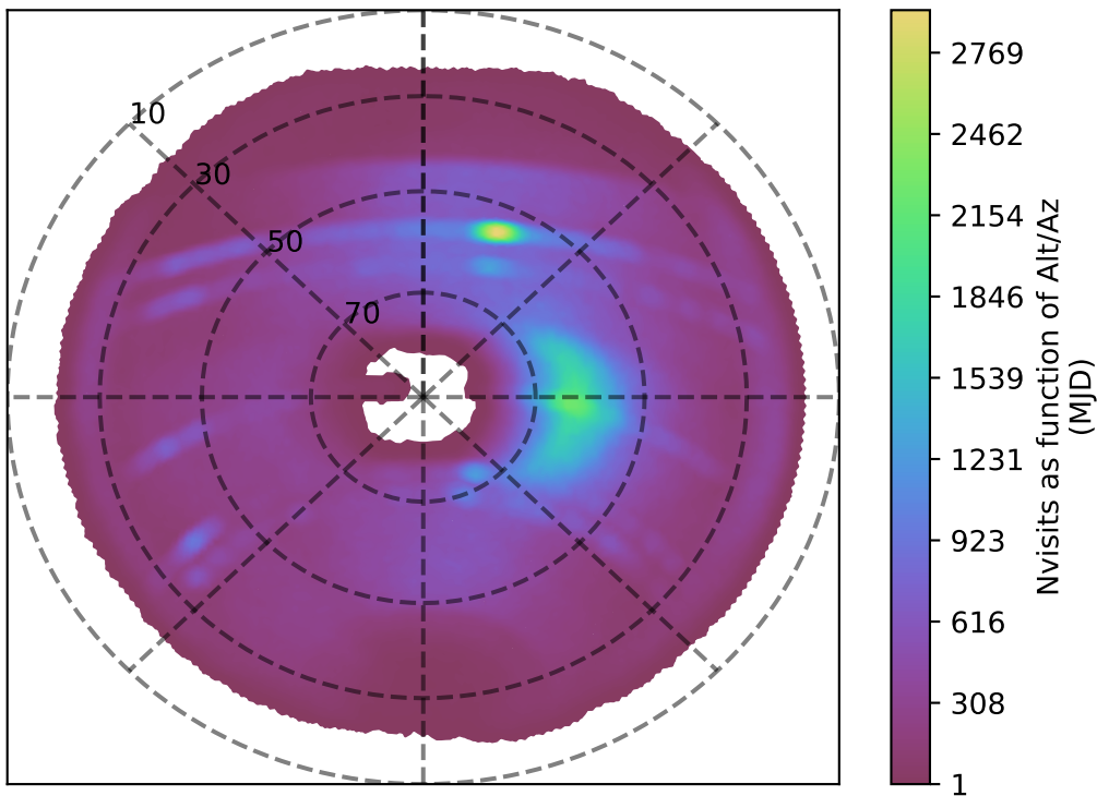
weather_cloudso14v3.4_10yrs z band: Nvisits as function of Alt/Az
