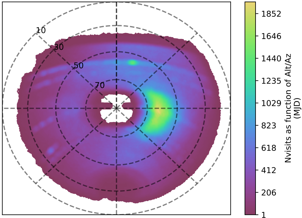
weather_cloudso14v3.4_10yrs y band: Nvisits as function of Alt/Az
