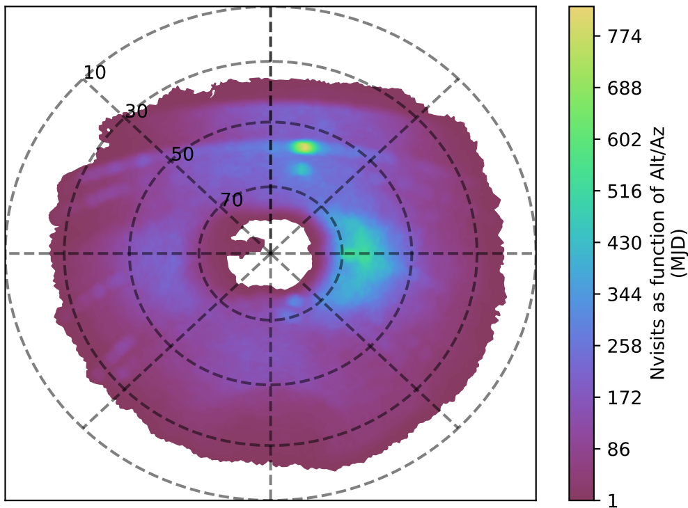
weather_cloudso14v3.4_10yrs u band: Nvisits as function of Alt/Az
